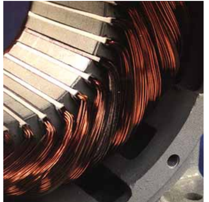
#8 Winding With Shorted Coil
