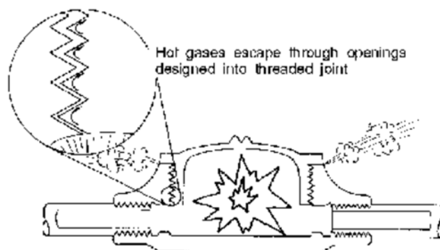
OPENINGS DESIGNED INTO THREADED JOINT
