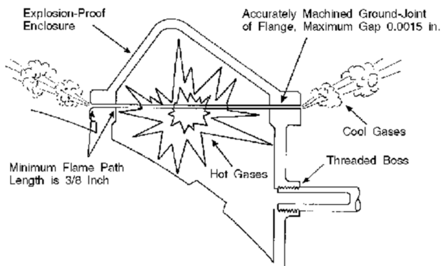
OPENINGS DESIGNED INTO GROUND JOINT
