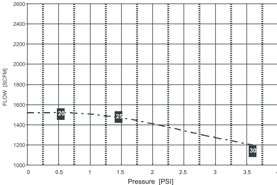
HIGH FLOW MODEL PRESSURE DATA CURVES ± 10%
